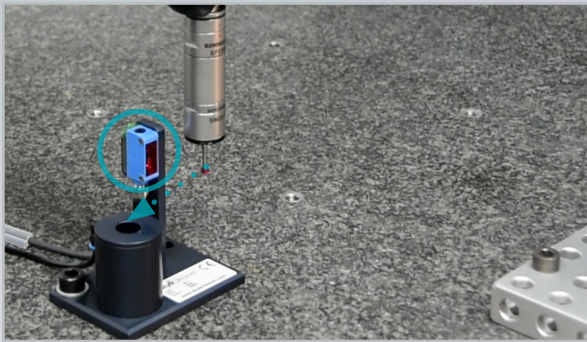
1. The stylus moves along the activation sensor. This starts the cleaning cycle
